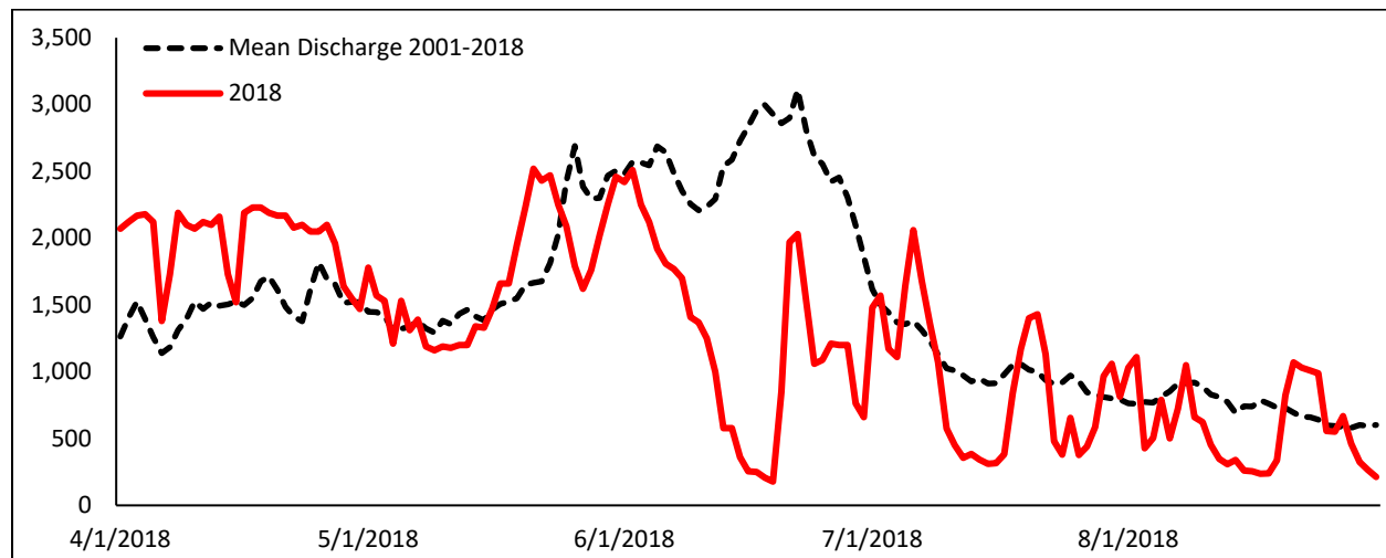
Figure 2. Mean daily discharge (ft 3 /second; cfs) at Kearney, Nebraska (USGS gage 06770200). Average across 2001–2018 from Kearney (USGS gage 06770200). See Figure 3 for the location of gage stations within our study area. Data available at:
