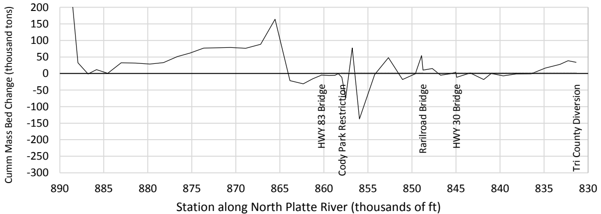
Figure A-7 Spatial Results, Run 3 Alt C Channel Widening U/S HWY 83 2009 – 2014 Hydrology – Channel Profile at Start and End (top), Change in Channel Invert Elevation (middle), and Cumulative Mass Bed Change (bottom).
