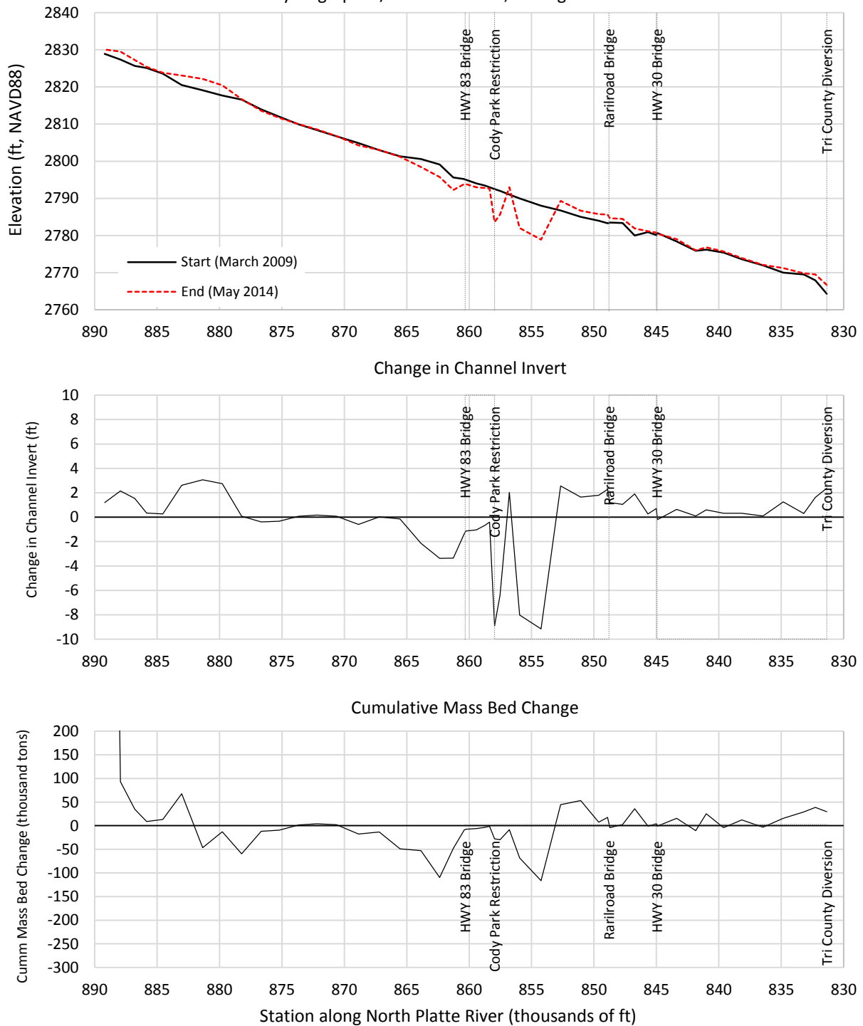
Channel Widening U/S HWY 83 + Jetties and Dredging D/S of HWY 83 16-Year Hydrograph w/ Flood & SDHFs, Change in Channel Profile
