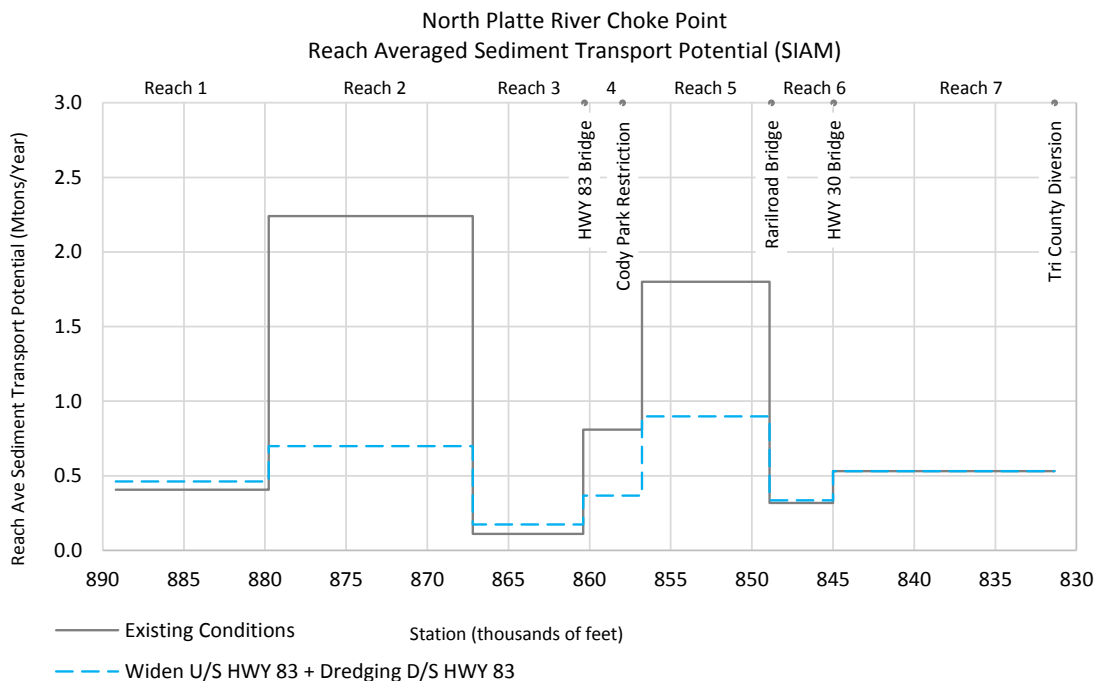
Figure 11. North Platte River Choke Point Reach-Averaged Sediment Transport Potential, Existing vs Alternative D (Widening U/S HWY 83 + Dredging D/S HWY 83).
