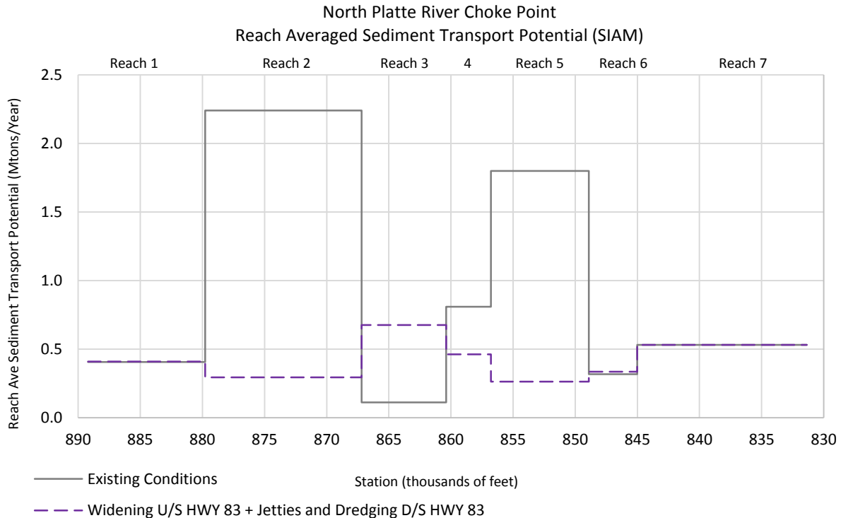
Figure 17. North Platte River Choke Point Reach-Averaged Sediment Transport Potential, Existing vs Alternative D (Widening U/S HWY 83 + Jetties and Dredging D/S HWY 83).
