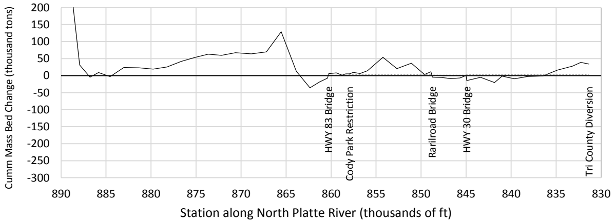
Figure A-10 Spatial Results, Run 4 (Alt D) Channel Widening U/S HWY 83 + Dredging D/S HWY 83 2009 – 2014 Hydrology – Channel Profile at Start and End (top), Change in Channel Invert Elevation (middle), and Cumulative Mass Bed Change (bottom).
