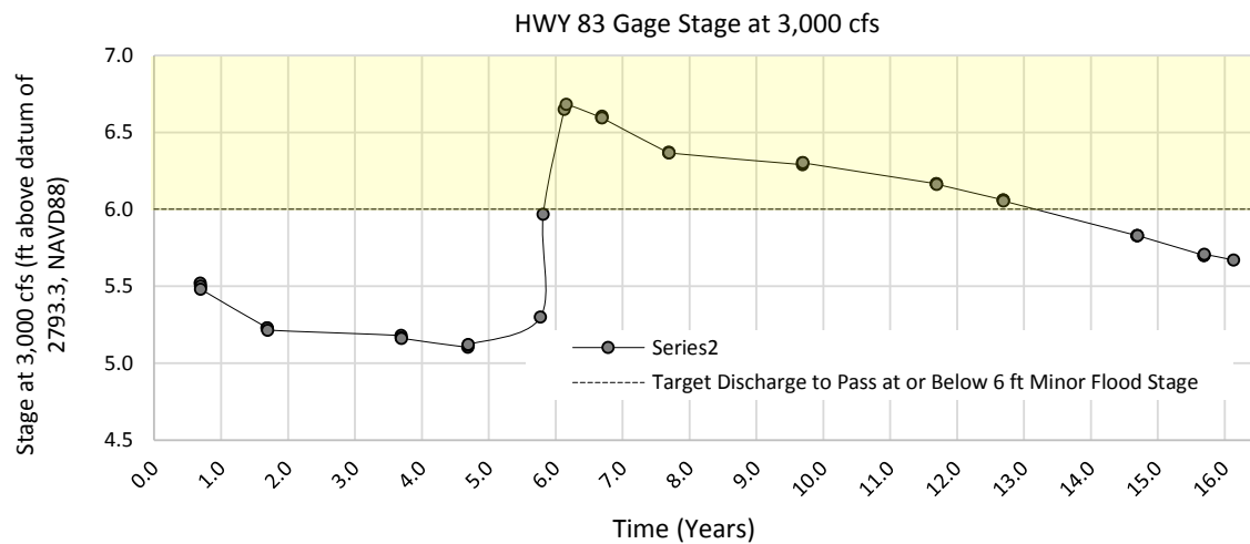
Figure A-15 Capacity at HWY 83 Gage through Time, Run 5 (Alt D) Channel Widening U/S HWY 83 + Dredging D/S HWY 83 16-year Hydrograph w/ Flood and SDHFs – 16-year Daily Discharge Hydrograph w/ Flood and SDHFs (top), Hydraulic Capacity at Minor Flood Stage (middle), and Stage at 3,000 cfs (bottom).
