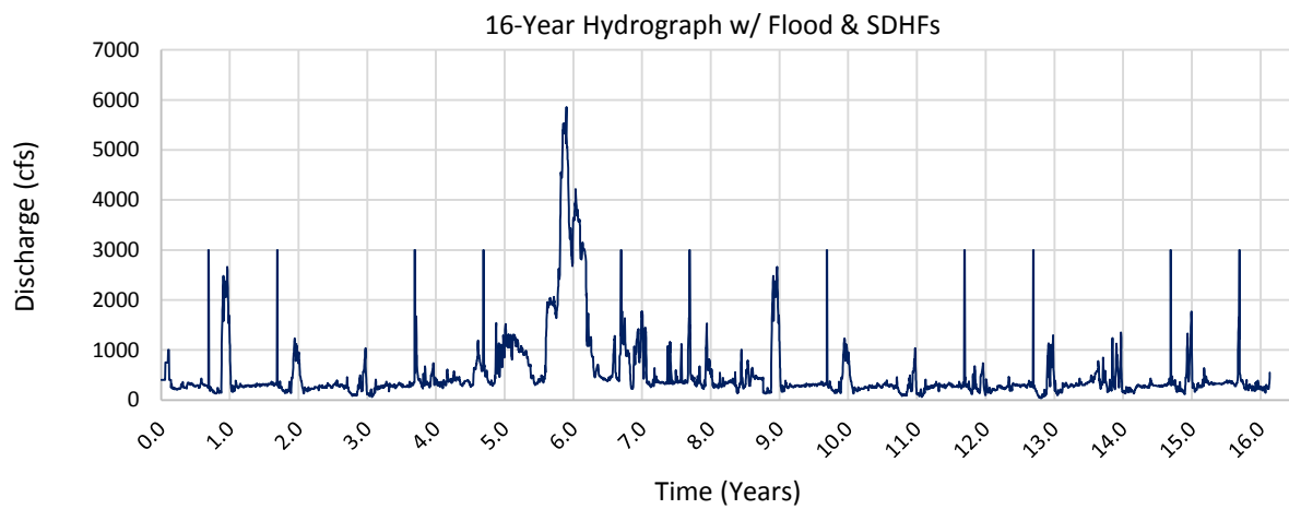
Figure A-18 Results through Time, Run 6 (Alt E) Channel Widening U/S HWY 83 + Jetties and Dredging D/S HWY 83 16-year Hydrograph w/ Flood and SDHFs - Channel Invert and Water Surface Elevation at the HWY 83 Gage (top), 16-year Daily Discharge Hydrograph w/ Flood and SDHFs (bottom).
