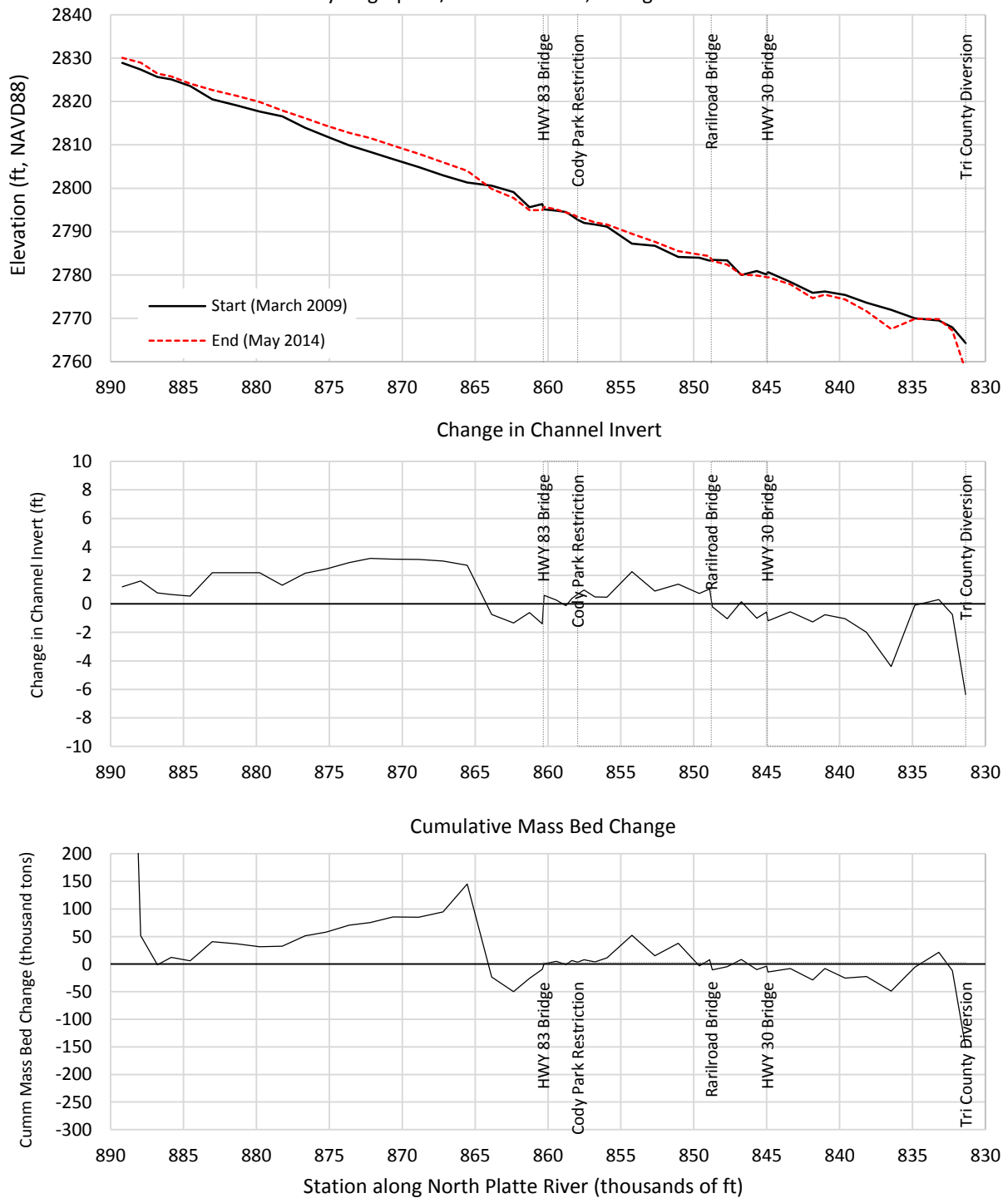
Figure A-13 Spatial Results, Run 5 (Alt D) Channel Widening U/S HWY 83 + Dredging D/S HWY 83 16-year Hydrograph w/ Flood and SDHFs – Channel Profile at Start and End (top), Change in Channel Invert Elevation (middle), and Cumulative Mass Bed Change (bottom).
