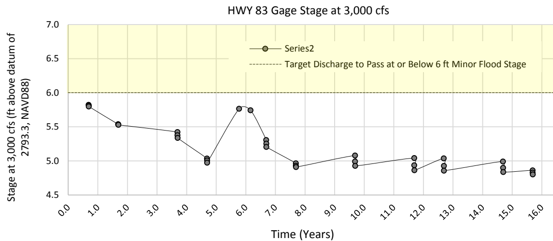
Figure A-19 Capacity at HWY 83 Gage through Time, Run 6 (Alt E) Channel Widening U/S HWY 83 + Jetties and Dredging D/S HWY 83 16-year Hydrograph w/ Flood and SDHFs – 16-year Daily Discharge Hydrograph w/ Flood and SDHFs (top), Hydraulic Capacity at Minor Flood Stage (middle), and Stage at 3,000 cfs (bottom).
