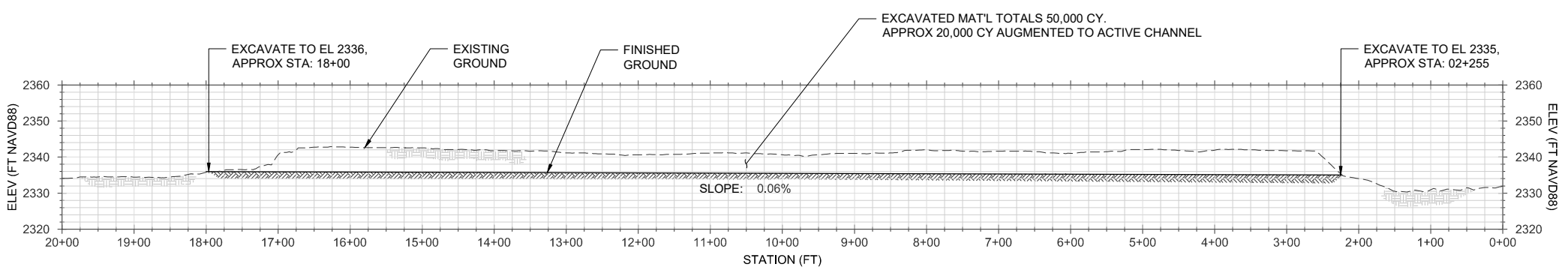
PILOT CHANNEL - PROFILE 1 H: 1 IN = 200 FT, V: 1 IN = 40
