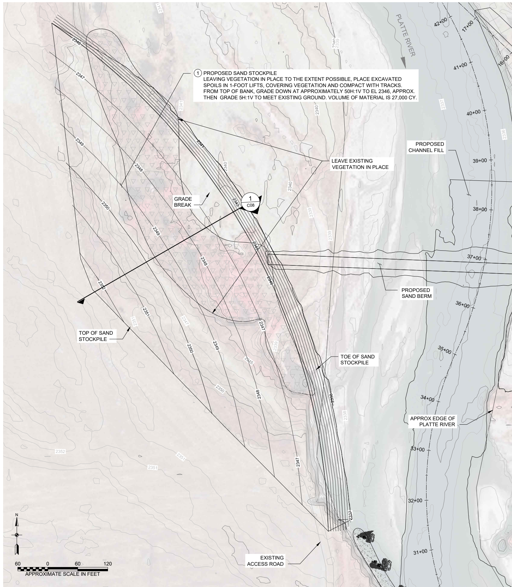
SAND STOCKPILE PLAN 1
