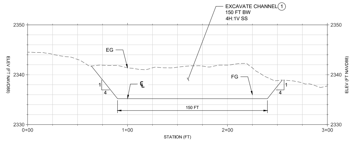
PILOT CHANNEL - CROSS SECTION H: 1 IN = 60 FT | V: 1 IN = 12 FT
