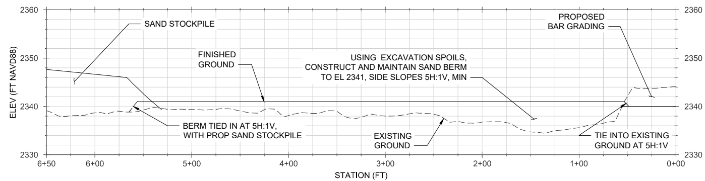
SAND BERM - PROFILE
