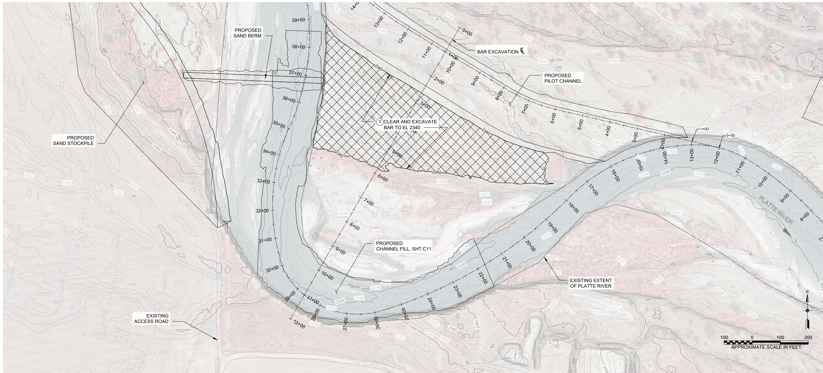
BAR GRADING - PLAN 1 -
