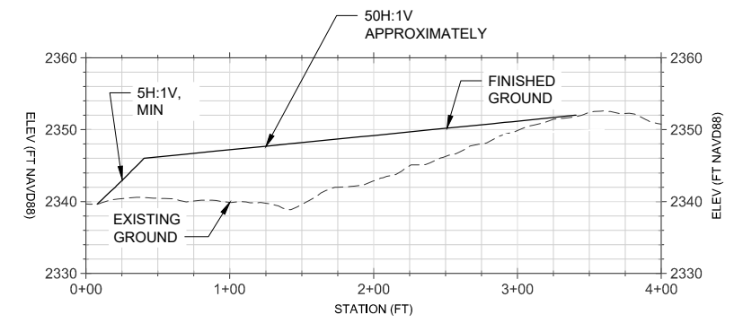
SAND STOCKPILE - CROSS SECTION 1 H: 1 IN = 120 FT | V: 1 IN = 24 FT
