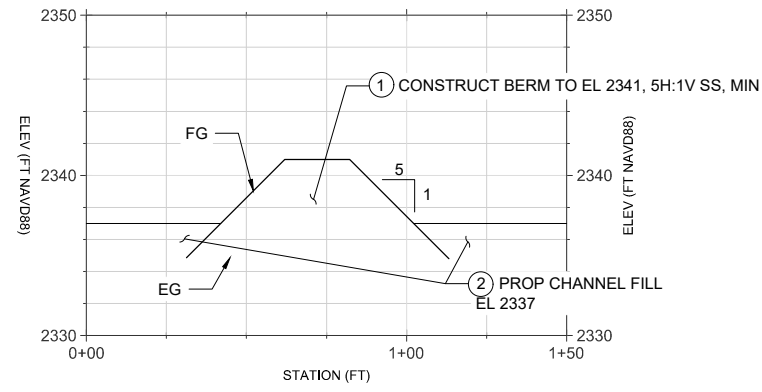
PILOT CHANNEL - CROSS SECTION 1 H: 1 IN = 60 FT | V: 1 IN = 12 FT C03
