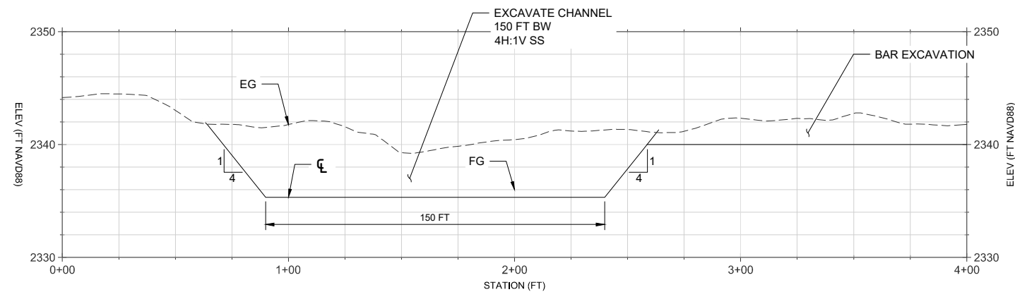
PILOT CHANNEL - CROSS SECTION H: 1 IN = 60 FT | V: 1 IN = 12 FT
