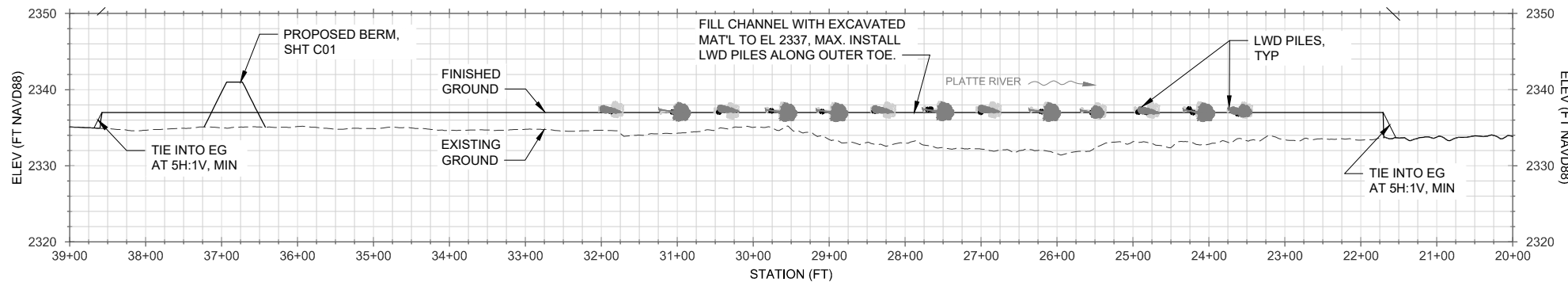
CHANNEL FILL - PROFILE H: 1 IN = 200 FT | V: 1 IN = 20 FT 1
