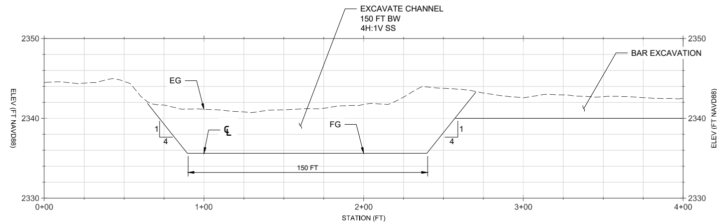
PILOT CHANNEL - CROSS SECTION H: 1 IN = 60 FT | V: 1 IN = 12 FT
