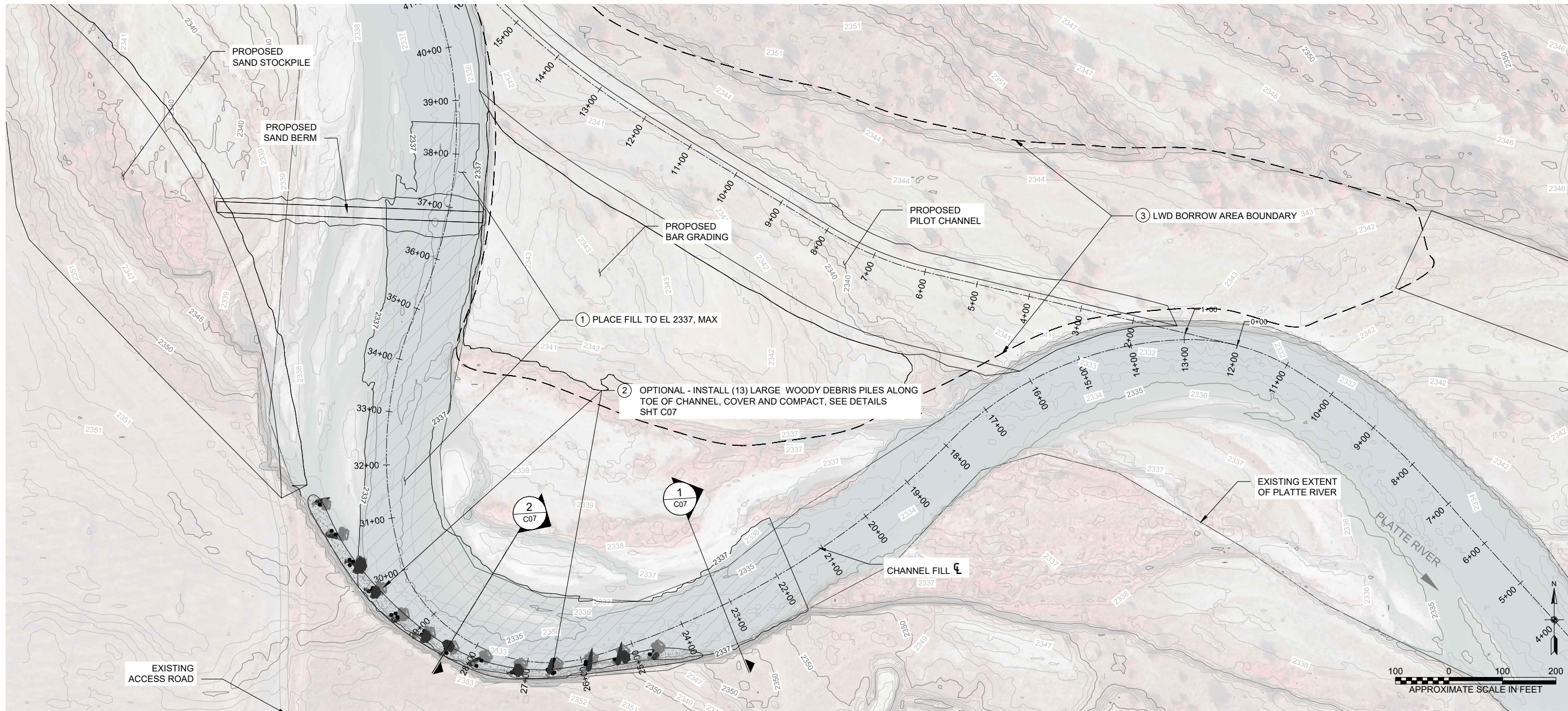
CHANNEL FILL - PLAN 1
