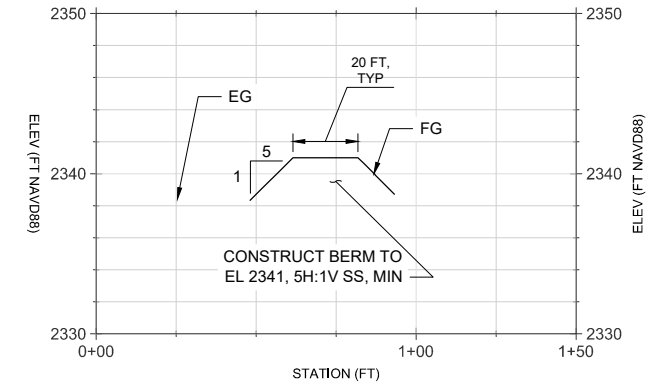
PILOT CHANNEL - CROSS SECTION 2 H: 1 IN = 60 FT | V: 1 IN = 12 FT C03
