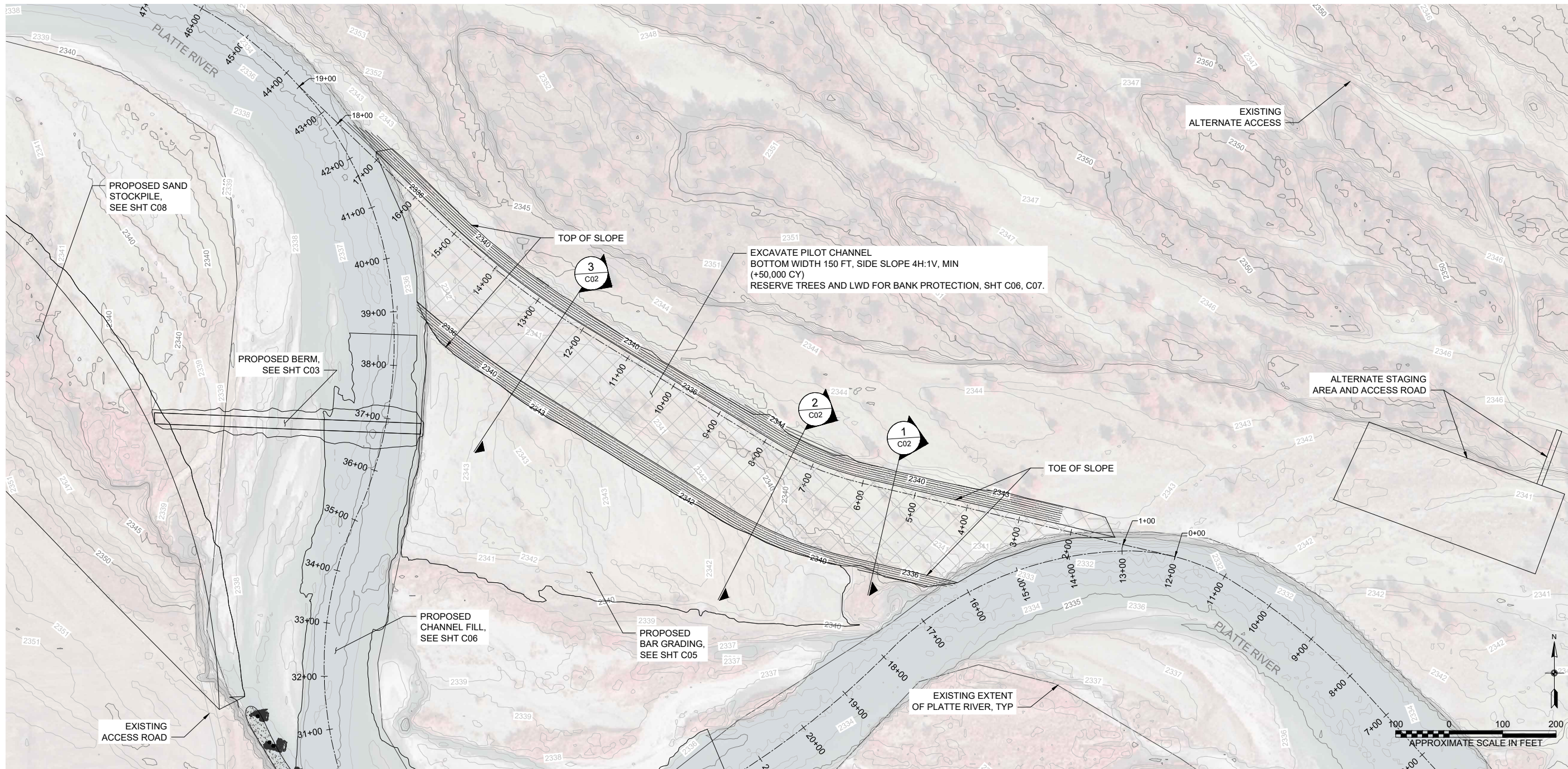
PILOT CHANNEL - PLAN 1
