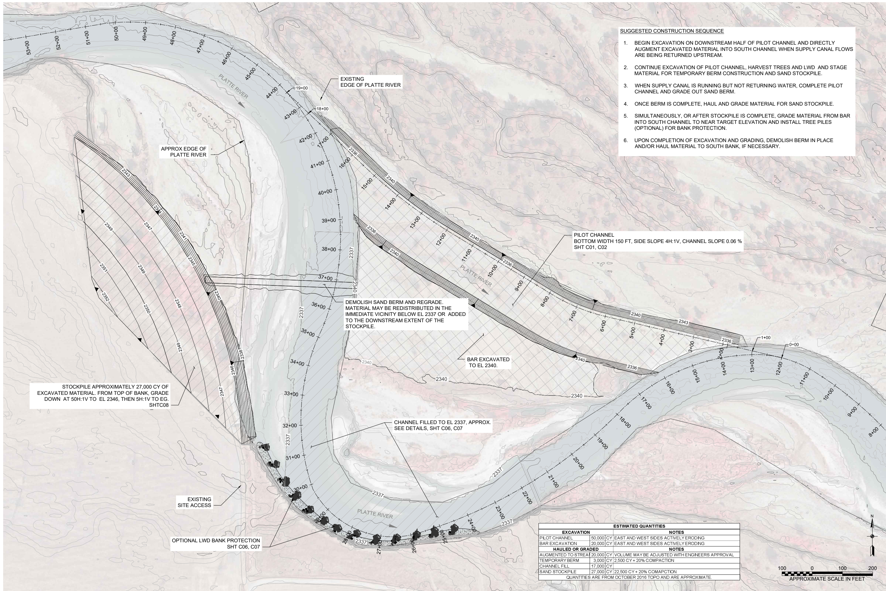
SITE PLAN SCALE: 1 IN = 200 FT
