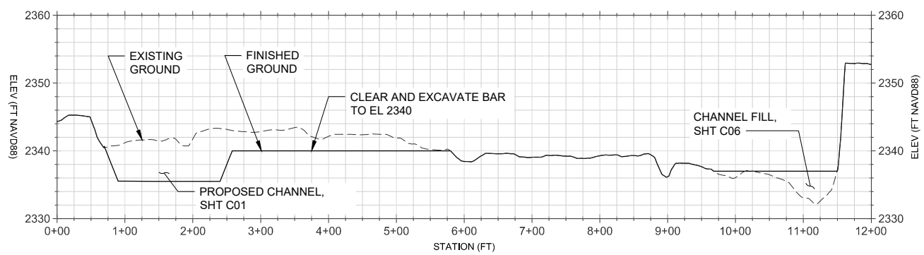
BAR GRADING - PROFILE H: 1 IN = 200 FT | V: 1 IN = 20 FT 1 -
