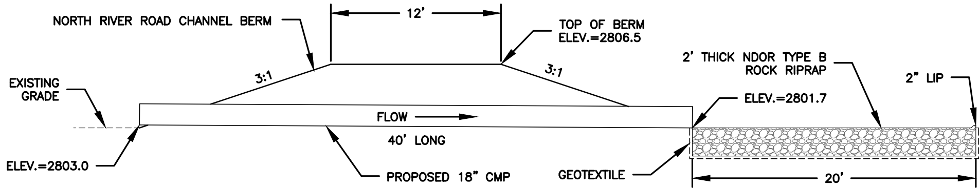
1 3/6 BERM CROSSING NORTH RIVER ROAD CHANNEL - CROSS SECTION NOT TO SCALE
