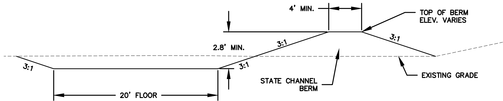
3 3/6 STATE CHANNEL - CROSS SECTION NOT TO SCALE
