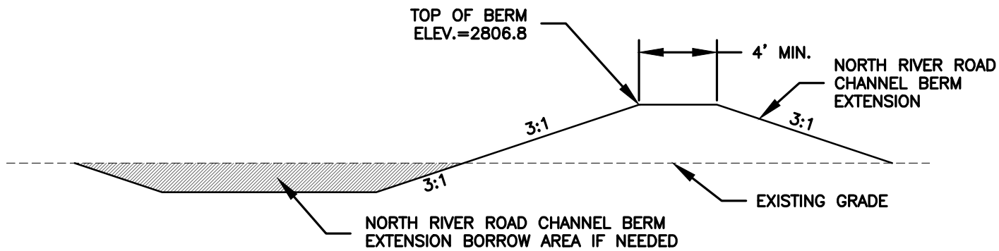
2 3/6 BERM EXTENSION NORTH RIVER ROAD CHANNEL - CROSS SECTION NOT TO SCALE
