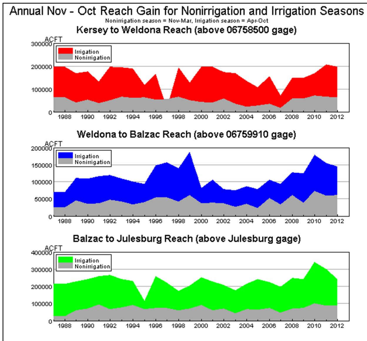
Figure 40. Calculated Annual Gain Summary in AF for the period of 1987-2012 Showing Irrigation and Off-Season Gain by Reach.
