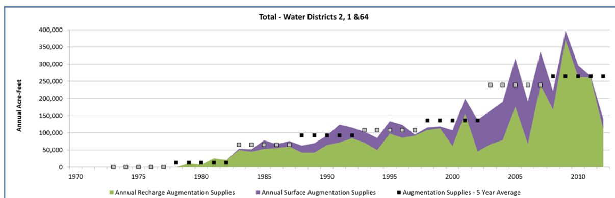
Figure 18. Total Annual Surface and Groundwater Supplies Used to Meet Estimated Potential Augmentation Requirements, and Five-Year Average Augmentation Supplies in Water Districts 2, 1 and 64. Data Source: CO DWR HydroBase Version 20130710.
