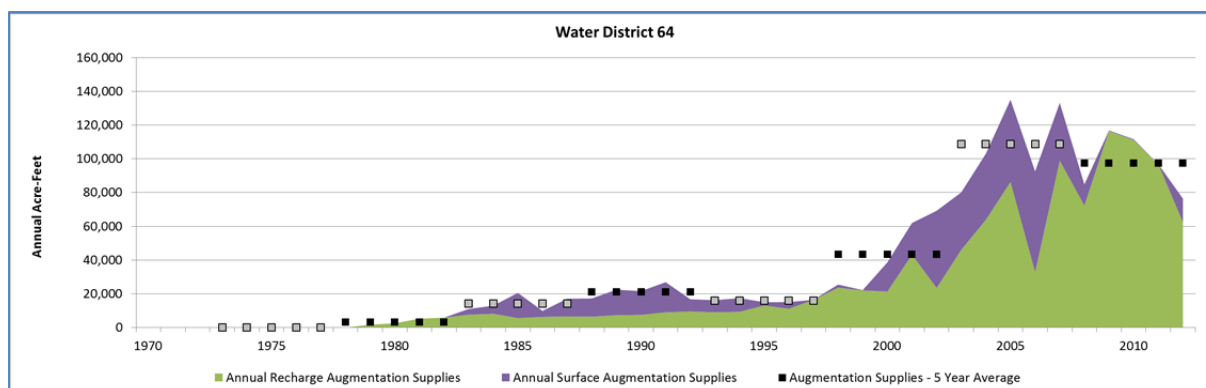
Figure 17. Annual Surface and Groundwater Supplies Used to Meet Estimated Potential Augmentation Requirements, and Five-Year Average Augmentation Supplies in Water District 64. Data Source: CO DWR HydroBase Version 20130710.
