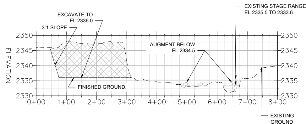
PILOT CHANNEL - PROFILE H: 1 IN = 200 FT, V: 1 IN = 20 FT
