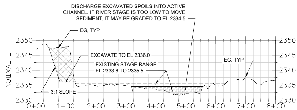
PILOT CHANNEL - PROFILE 3 H: 1 IN = 200 FT, V: 1 IN = 20 FT
