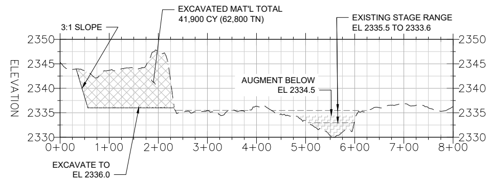
PILOT CHANNEL - PROFILE H: 1 IN = 200 FT, V: 1 IN = 20 FT
