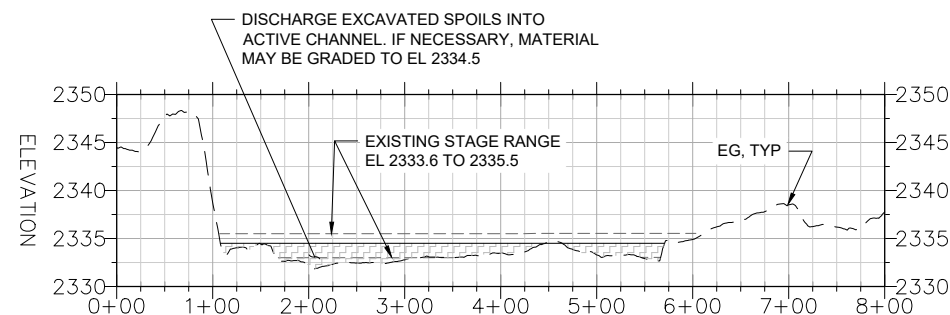
PILOT CHANNEL - PROFILE 4 H: 1 IN = 200 FT, V: 1 IN = 20 FT
