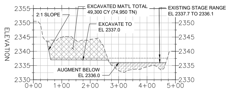
EXCAVATION - PROFILE 2 H: 1 IN = 100 FT, V: 1 IN = 10 FT
