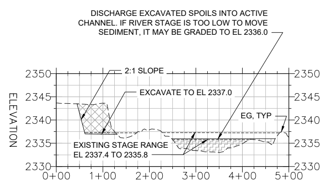
AUGMENTATION - PROFILE H: 1 IN = 100 FT, V: 1 IN = 10 FT
