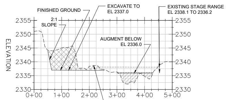
EXCAVATION - PROFILE 1 H: 1 IN = 100 FT, V: 1 IN = 10 FT
