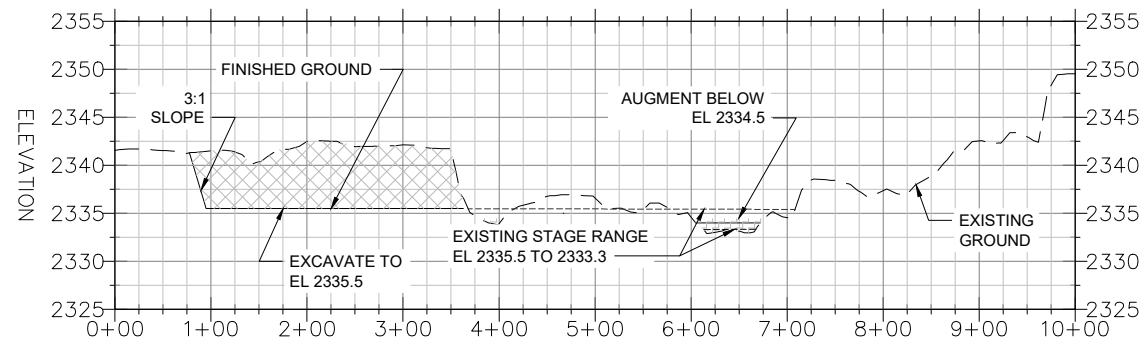
EXCAVATION - PROFILE 10X VERT. EXXAG.
