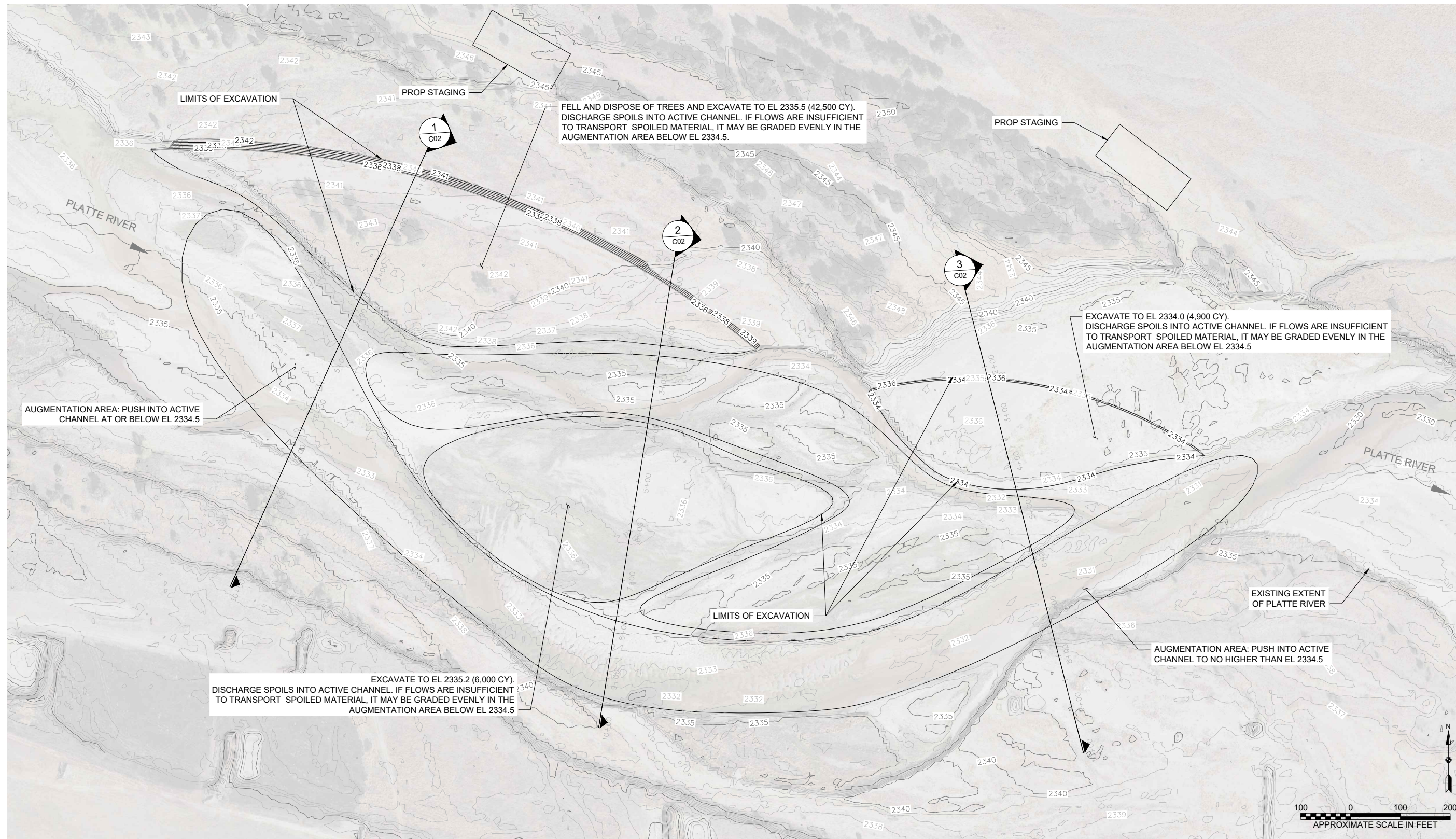
EXCAVATION AND AUGMENTATION - PLAN 1
